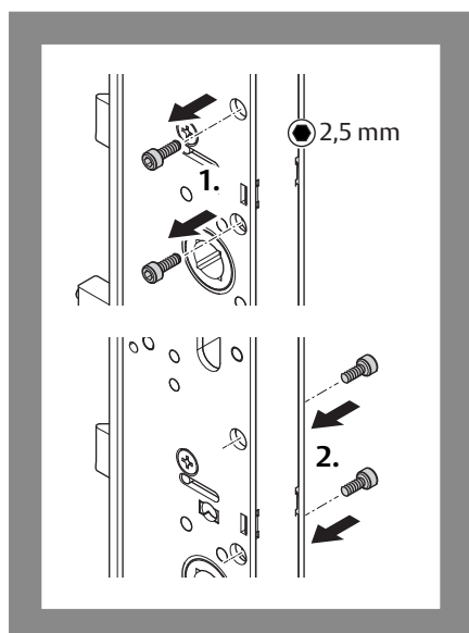
Fig. 12: Adjust the panic side
